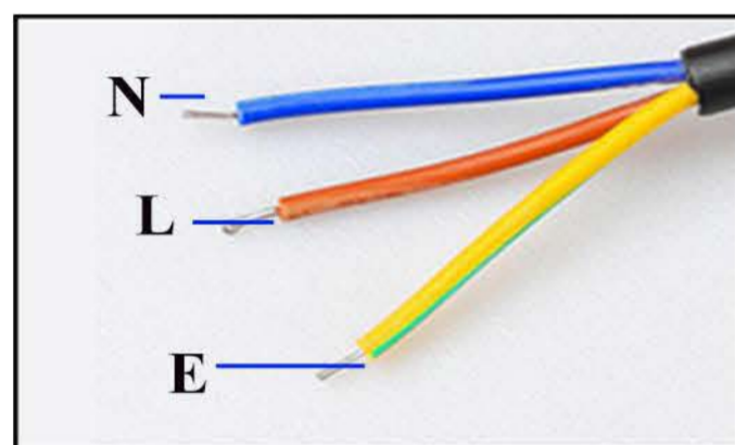
接线方法/Wiring method
