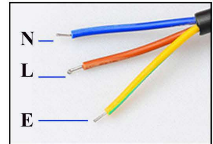
• 接线方法/Wiring method
